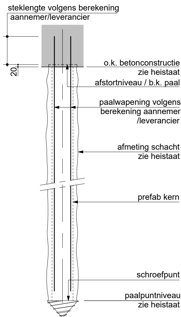
Principe detail Fundex-combipaal
